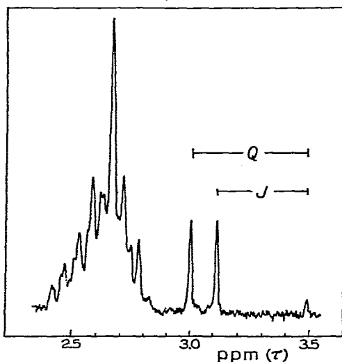
Fig. 2. PMR spectrum of ( \text{CH}_3 ) 3 SiCH=CHSi(C 6 H 5 ) 3 in \text{CCl}_4 . See text for assignments.
